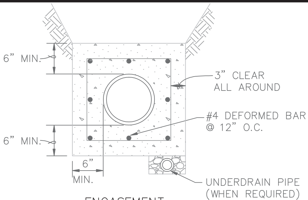
ENCASEMENT TYPICAL AND UNDERDRAIN
