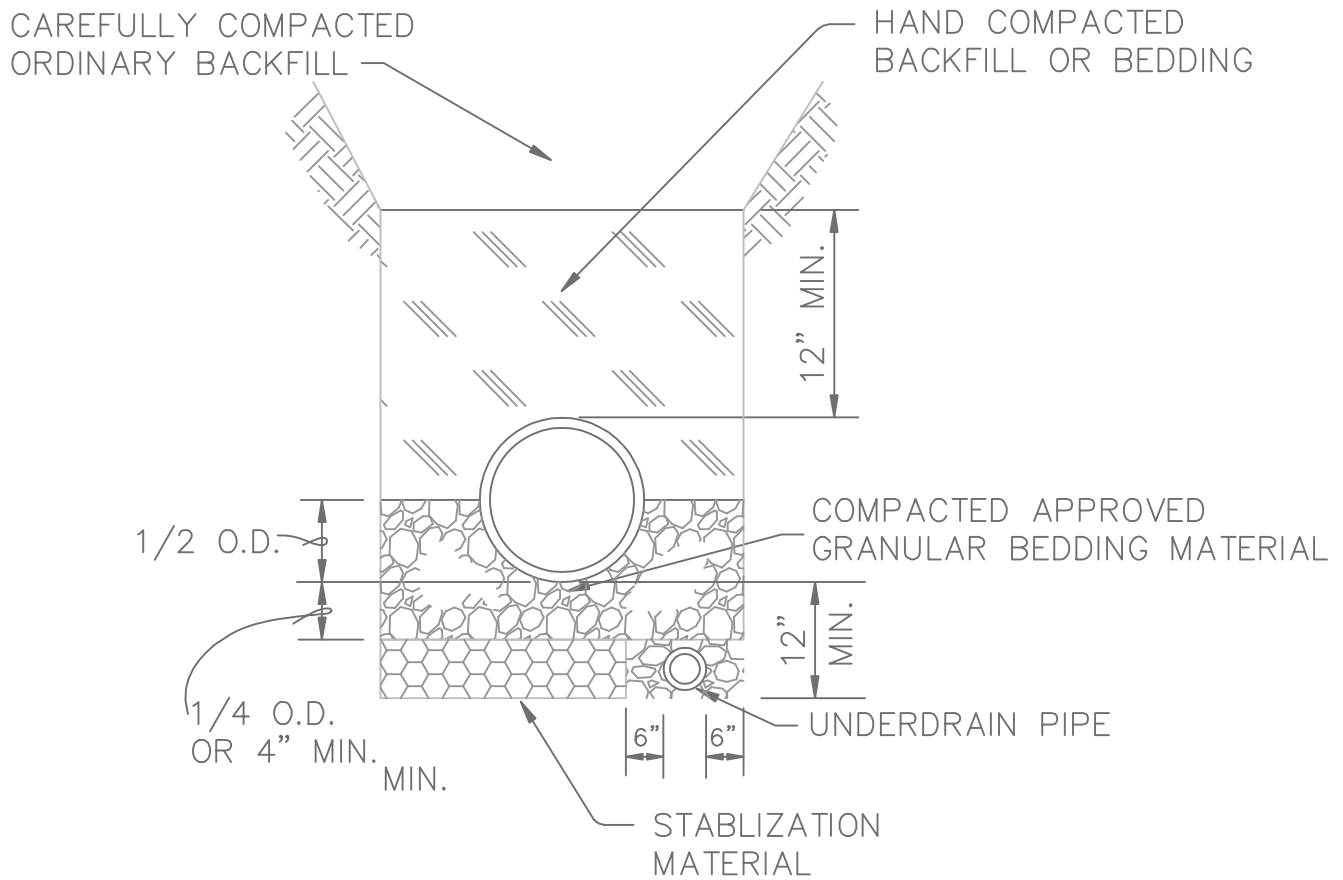
TYPICAL UNDERDRAIN
