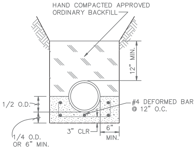
CLASS A CONCRETE CRADLE
