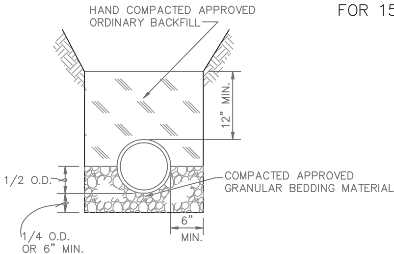
CLASS B COMPACTED GRANULAR BEDDING FOR 18" DIA. PIPE OR LARGER
