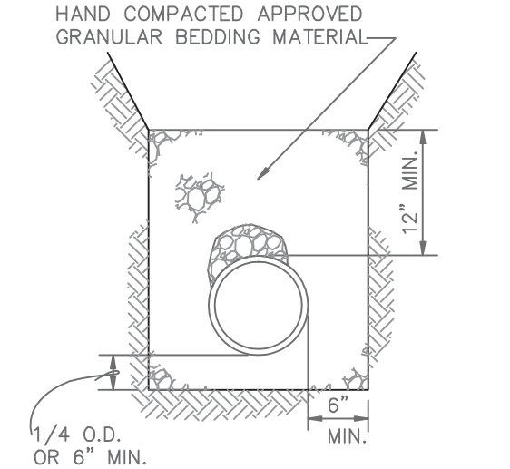
CLASS B COMPACTED GRANULAR BEDDING FOR 15" DIA. PIPE OR SMALLER
