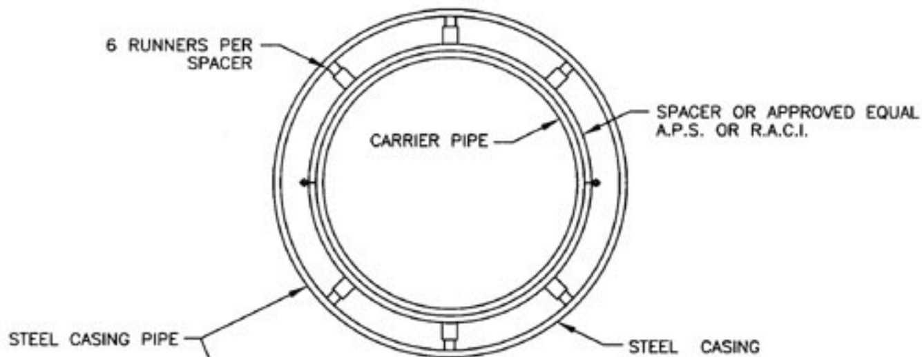
SECTION VIEW
