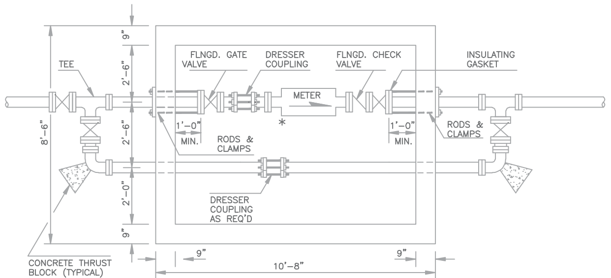
PLAN OF PIPING NO SCALE
