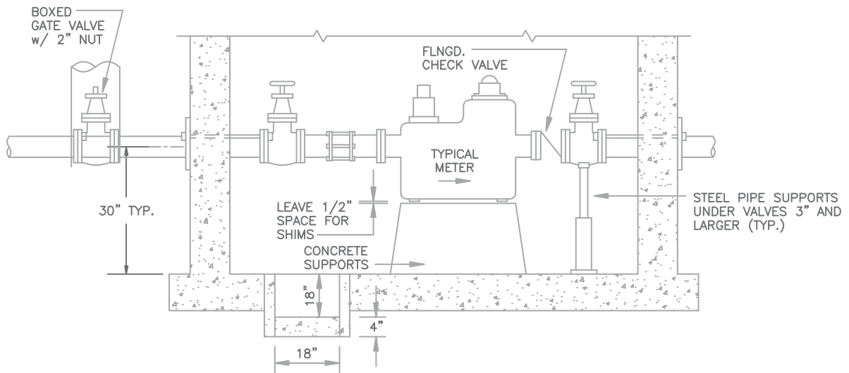
TYPICAL CONC. METER SUPPORTS NO SCALE
