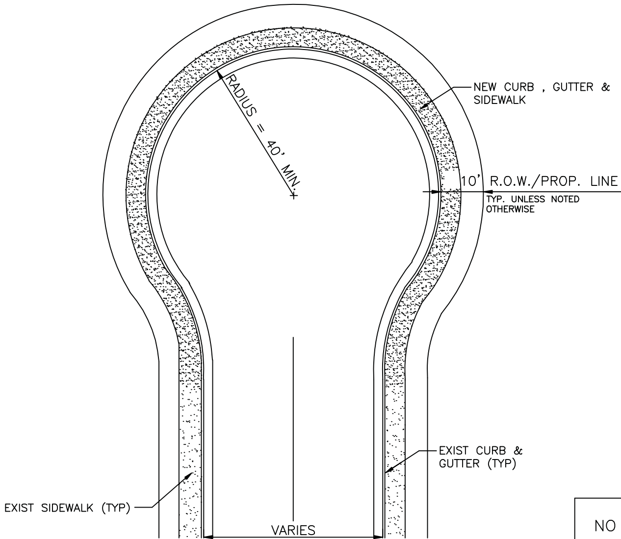
CUL-DE-SAC PLAN Not to Scale
