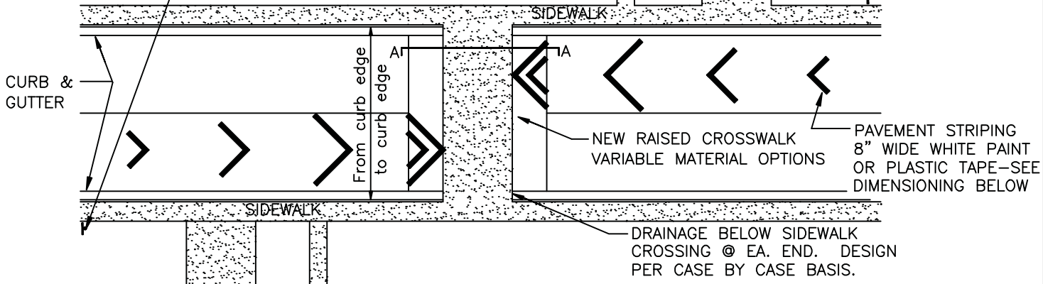
RAISED CROSSWALK PLAN Not to Scale
