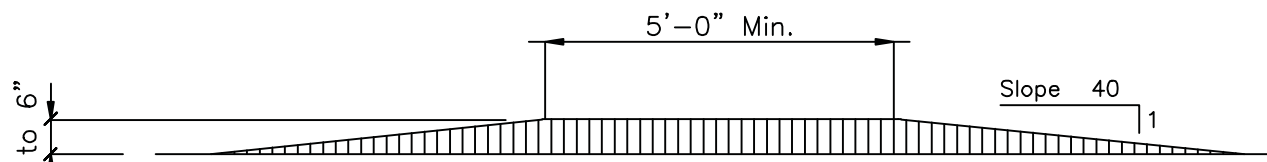
A-A RAISED CROSSWALK SECTION Not to Scale
