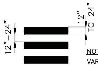
CROSSWALK STRIPING OPTION Not to Scale
