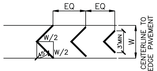
STRIPING DIMENSIONING Not to Scale
