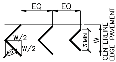
STRIPING MEASUREMENTS
