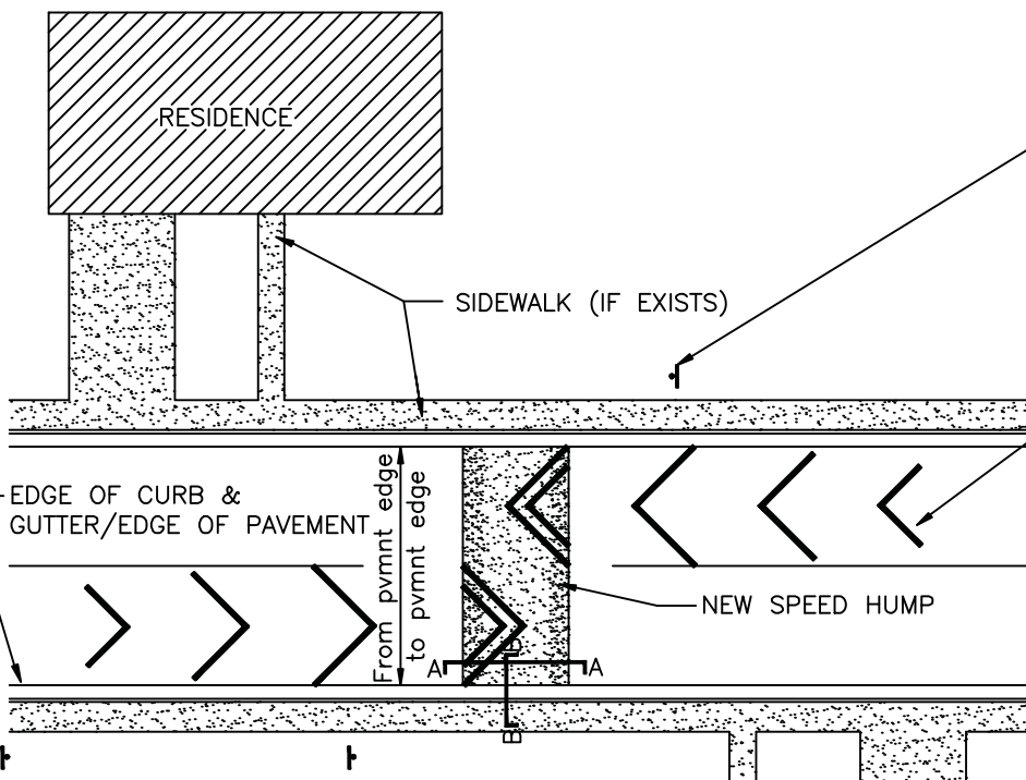
SPEED HUMP PLAN Not to Scale
